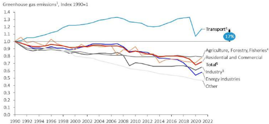
FIGURE 2 Evolution of greenhouse gas emissions by sector in the EU
